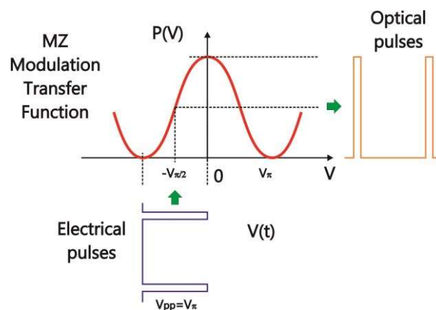
Pulse electrical signal with V\pi peak-to-peak voltage applied to a modulator to generate optical pulses with high extinction
