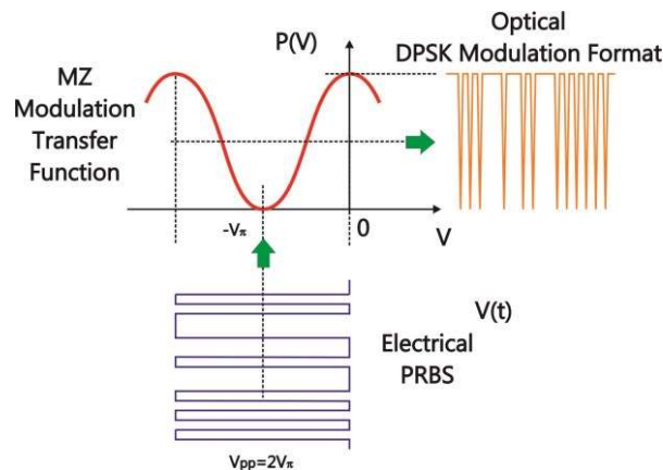
Electrical 20 Gb/s data stream with 2 \times V_{\pi} peak-to-peak voltage applied to a modulator to generate a high SNR 40 Gb/s DPSK optical data stream
