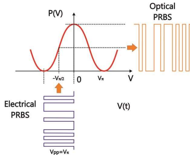
Electrical 10 Gb/s data stream with V_{\pi} peak-to-peak voltage applied to a modulator to generate a high SNR 10 Gb/s NRZ optical data stream
