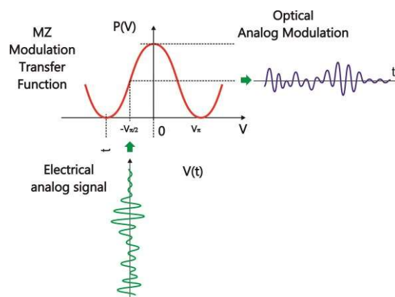
Electrical analog signal with < V_{\pi} peak-to-peak voltage applied to a modulator to generate a faithful optical reproduction
